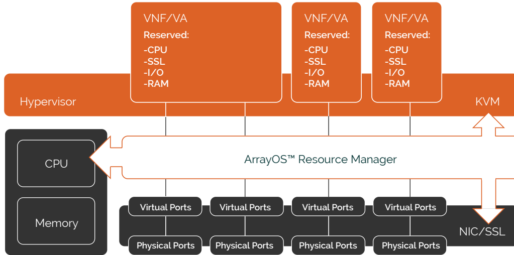
Figure 3: High-Level Network Functions Platform Architecture
